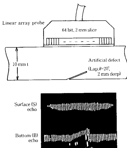
Fig. 5 An example of B scope projection (Scan mode: 8 bit group, 1 bit shift)
