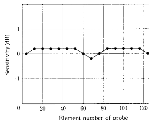
Fig. 7 Distribution of sensitivity in concurrent excitation of 8 elements
