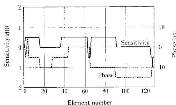
Fig. 6 Distribution of sensitivity and phase between sliced elements
