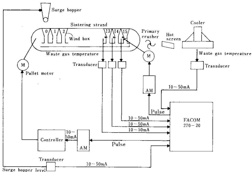
Fig. 8 Outline of sequence for strand speed control
