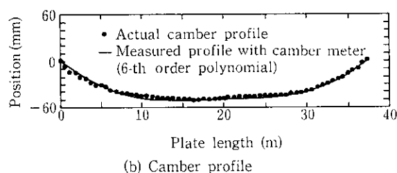
Fig. 4 An example of camber profile measurement
