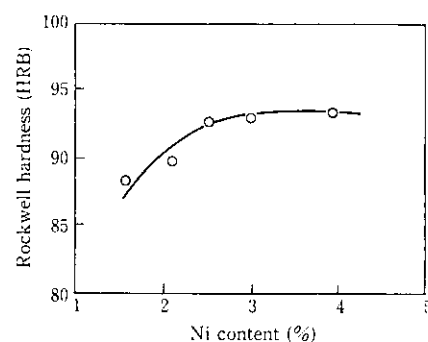
Fig. 3 Relationship between Ni content and Rockwell hardness for sintered compacts of 1%Mo containing composite-type alloyed steel powders with 0.6% graphite
